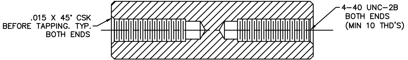
FULL SECTION VIEW
